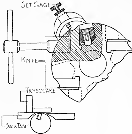
FIG. 141. TESTING JOINTER KNIVES FOR POSITION.
